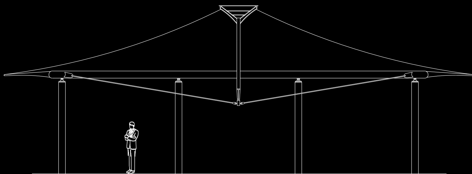
SECTION (12m MODULE)
